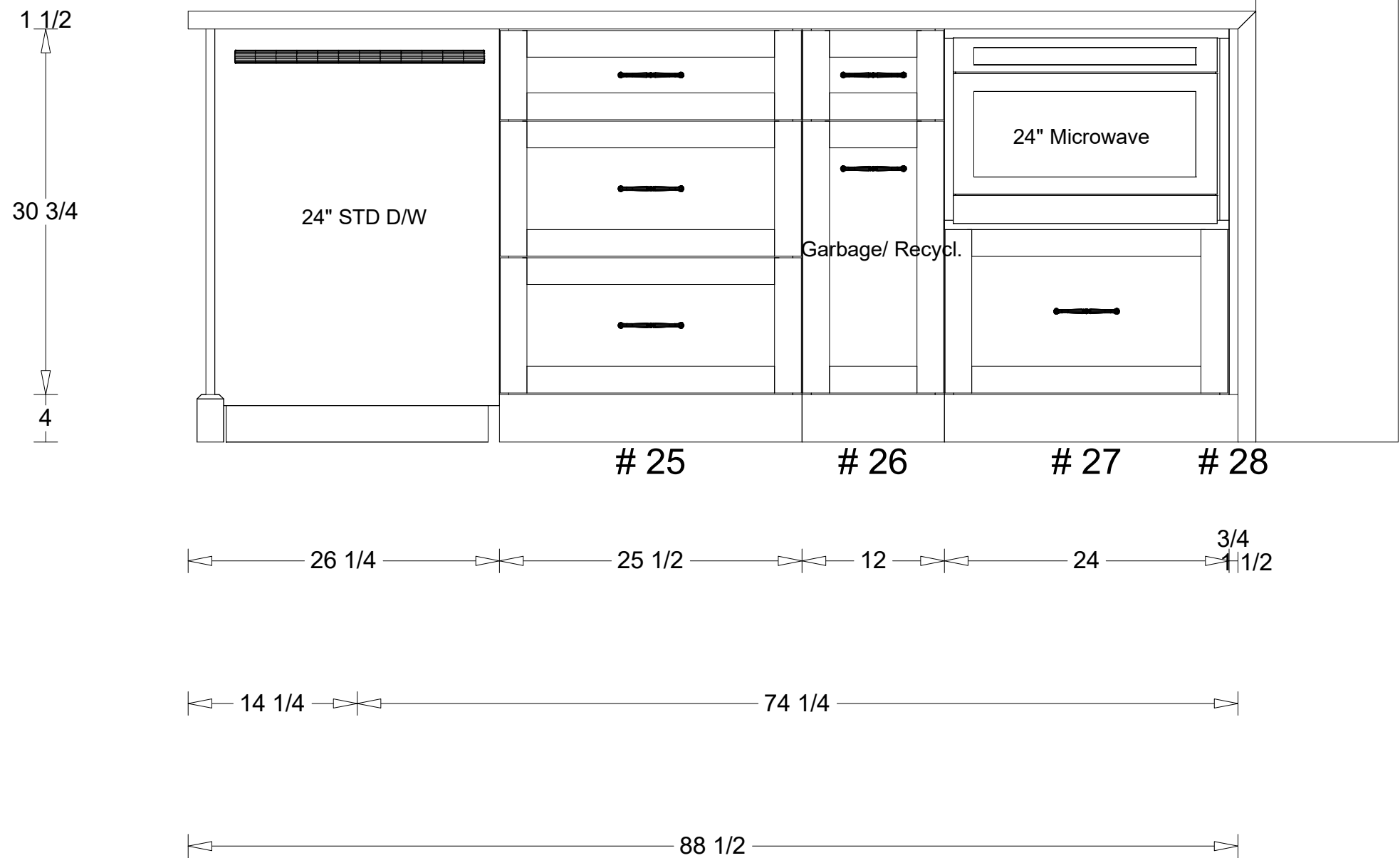
Island Front Elev.
