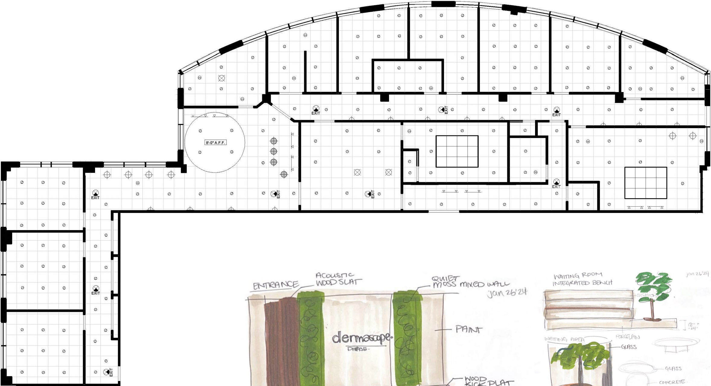
REFLECTED CEILING PLAN
